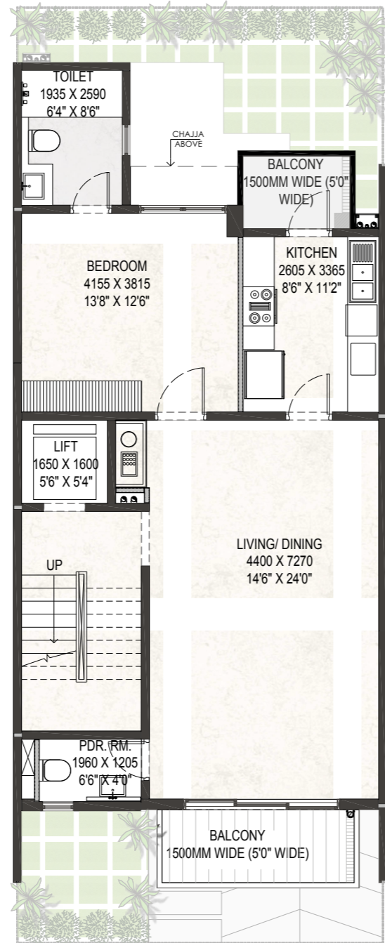
UPPER GROUND FLOOR PLAN
